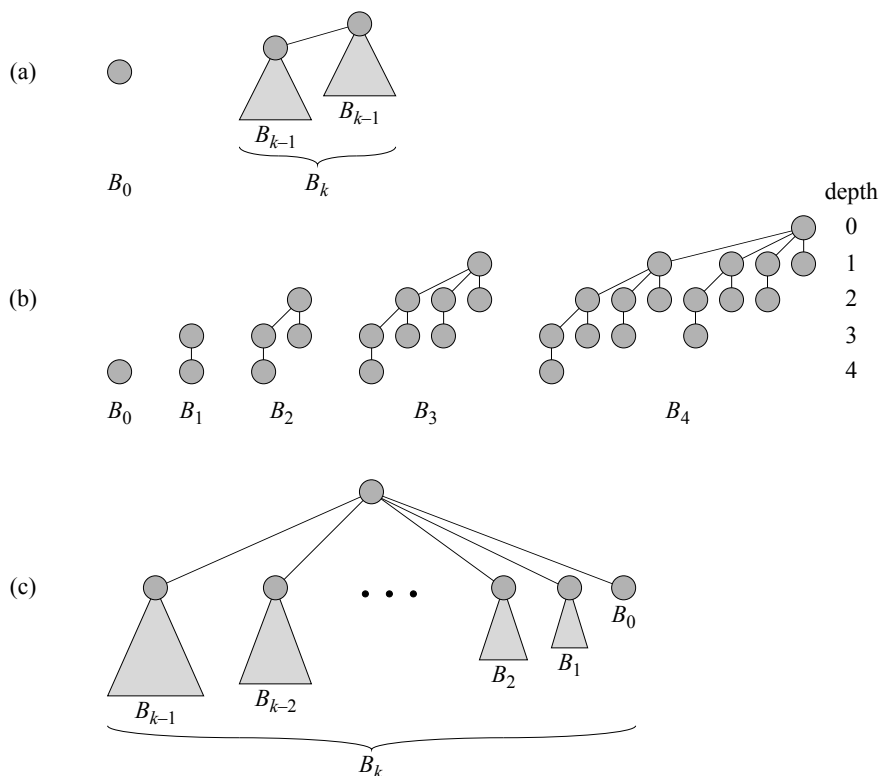
Figure 19.6 (a) The recursive definition of the binomial tree B_k . Triangles represent rooted sub-trees. (b) The binomial trees B_0 through B_4 . Node depths in B_4 are shown. (c) Another way of looking at the binomial tree B_k .
